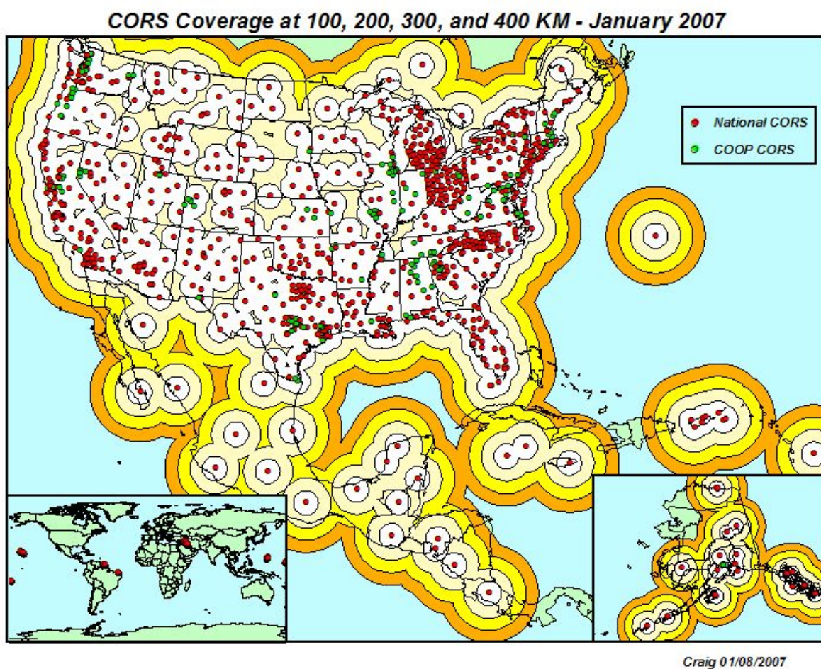
Figure B-14. CORS coverage as of January 2007
